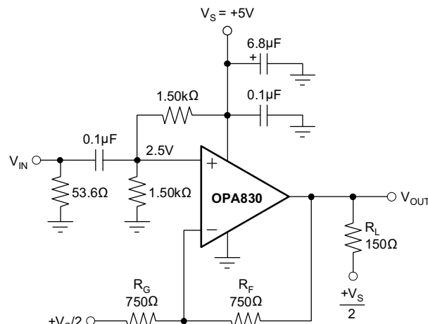
Figure 51. AC-Coupled, G = +2, +5V Single-Supply Specification and Test Circuit
